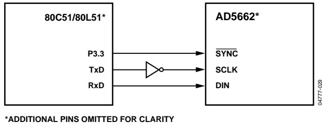
Figure 39. AD5662 to 80C51/80L51 Interface
