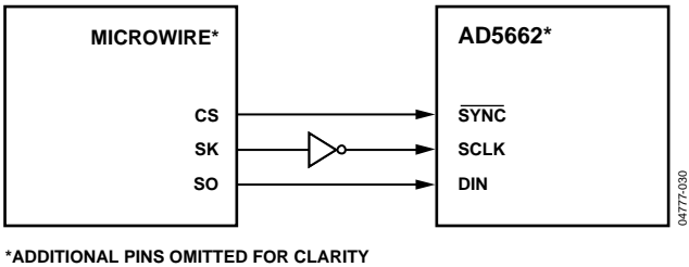
Figure 40. AD5662 to MICROWIRE Interface
