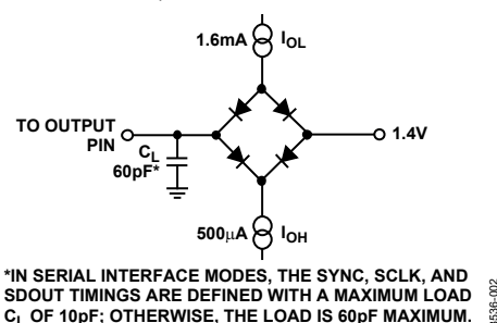
Figure 2. Load Circuit for Digital Interface Timing
