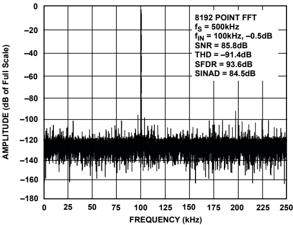
Figure 8. FFT Plot
